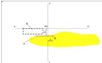
VOL headlight
