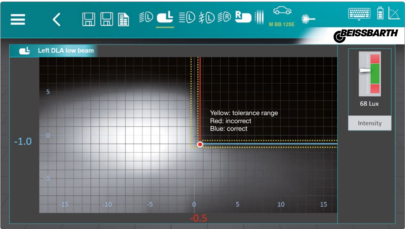
Adjustment of headlights with DLA high-beam assistant (test image control via vehicle ECU diagnosis)
