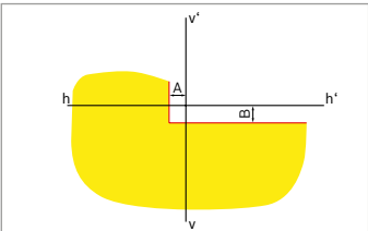
DLA-Scheinwerfer links
