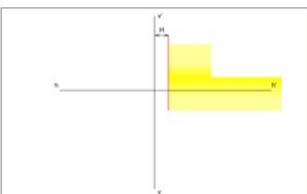
Škoda Kink Scheinwerfer links
